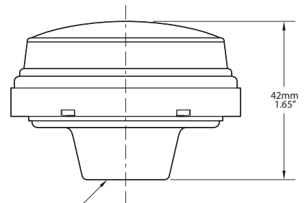
1" - 14 - UNS-2B Thread (1" - 14 TPI Standard Marine Mount)
