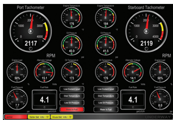
N2KView® Engine Screen
