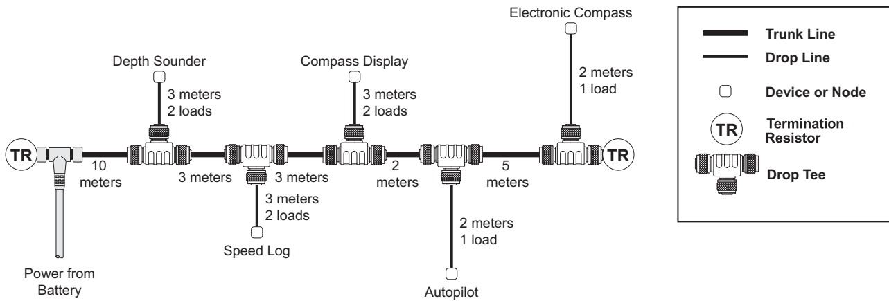
FIGURE 6. End-Powered Network
