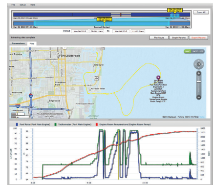
N2KExtractor® Screen Shot
