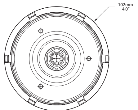
1" - 14 - UNS-2B Thread (1" - 14 TPI Standard Marine Mount)
